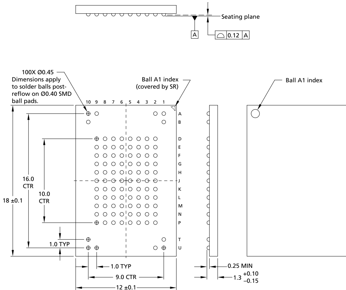
Figure 7: 100-Ball LBGA – 12mm x 18mm (Package Code: H3)
