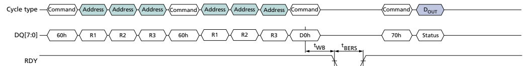
Figure 62: ERASE BLOCK MULTI-PLANE (60h-60h-D0h) Operation
