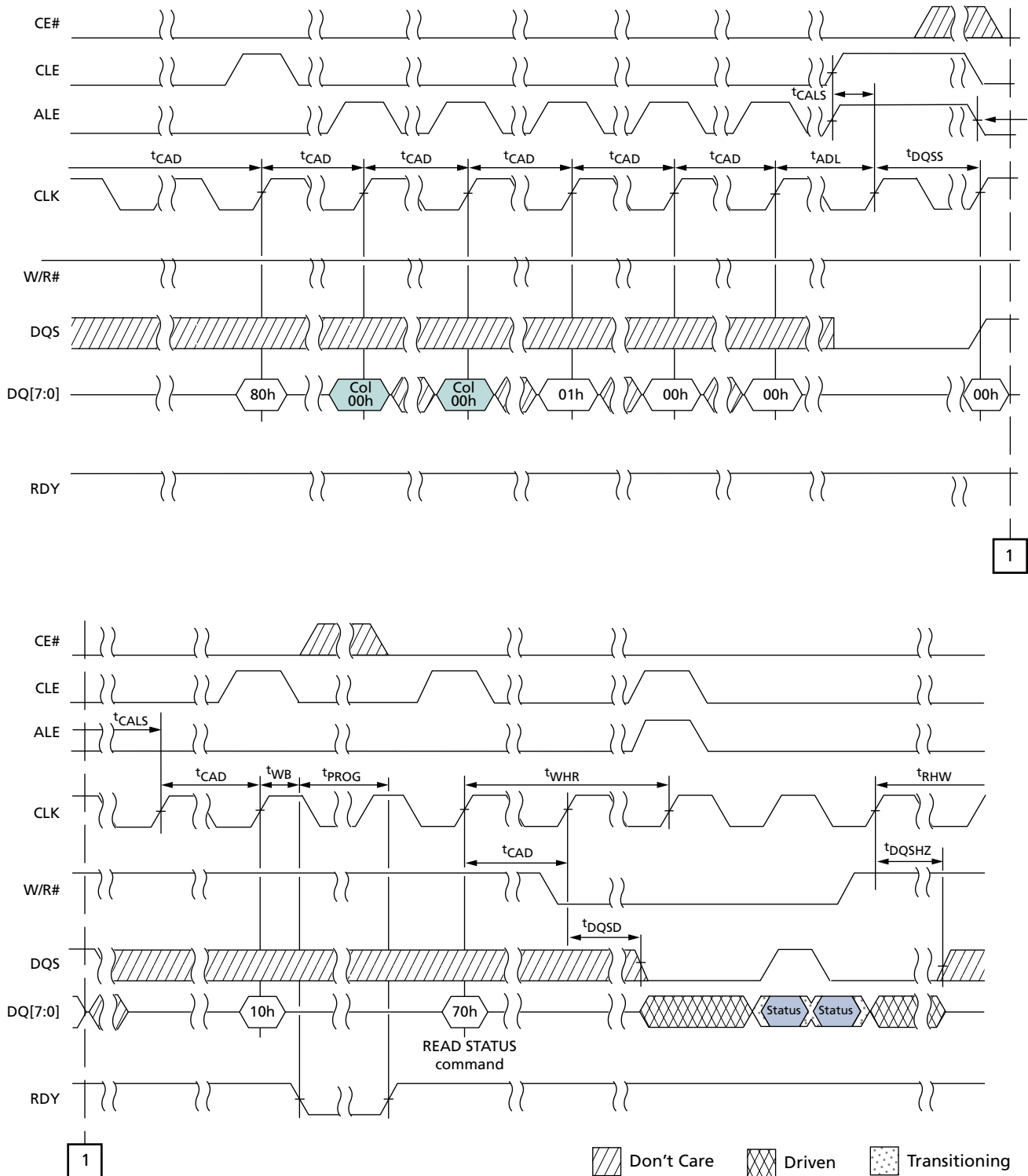
Figure 118: PROTECT OTP AREA
