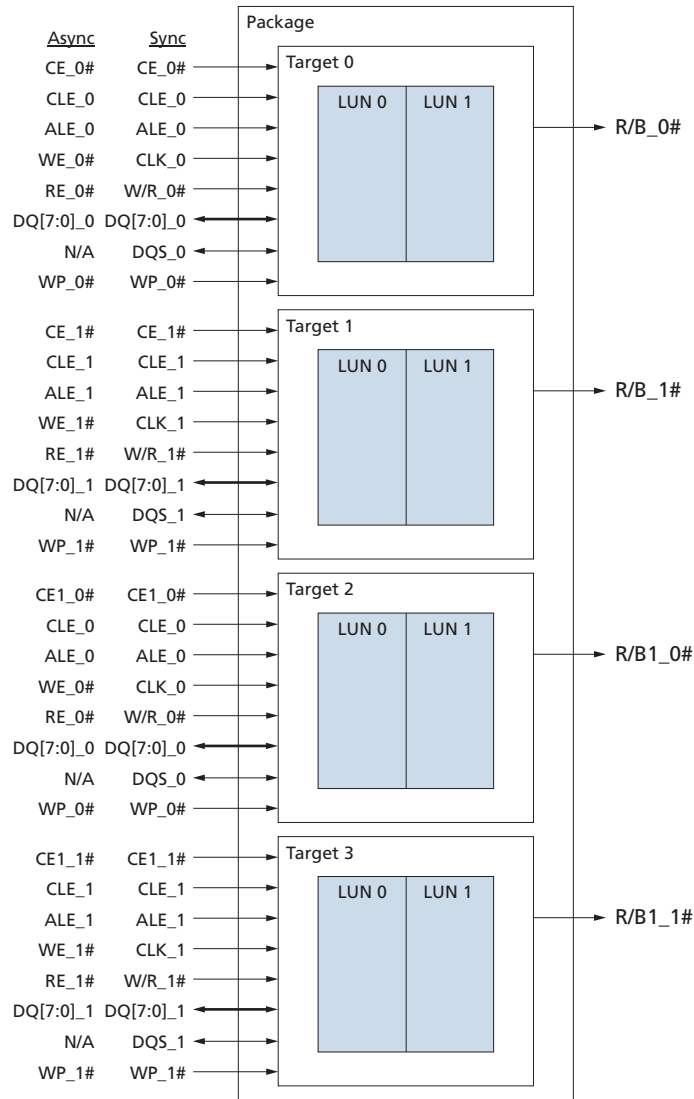
Figure 13: Device Organization for Eight-Die Package (BGA)
