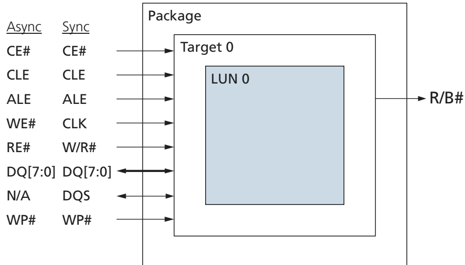
Figure 9: Device Organization for Single-Die Package (TSOP)
